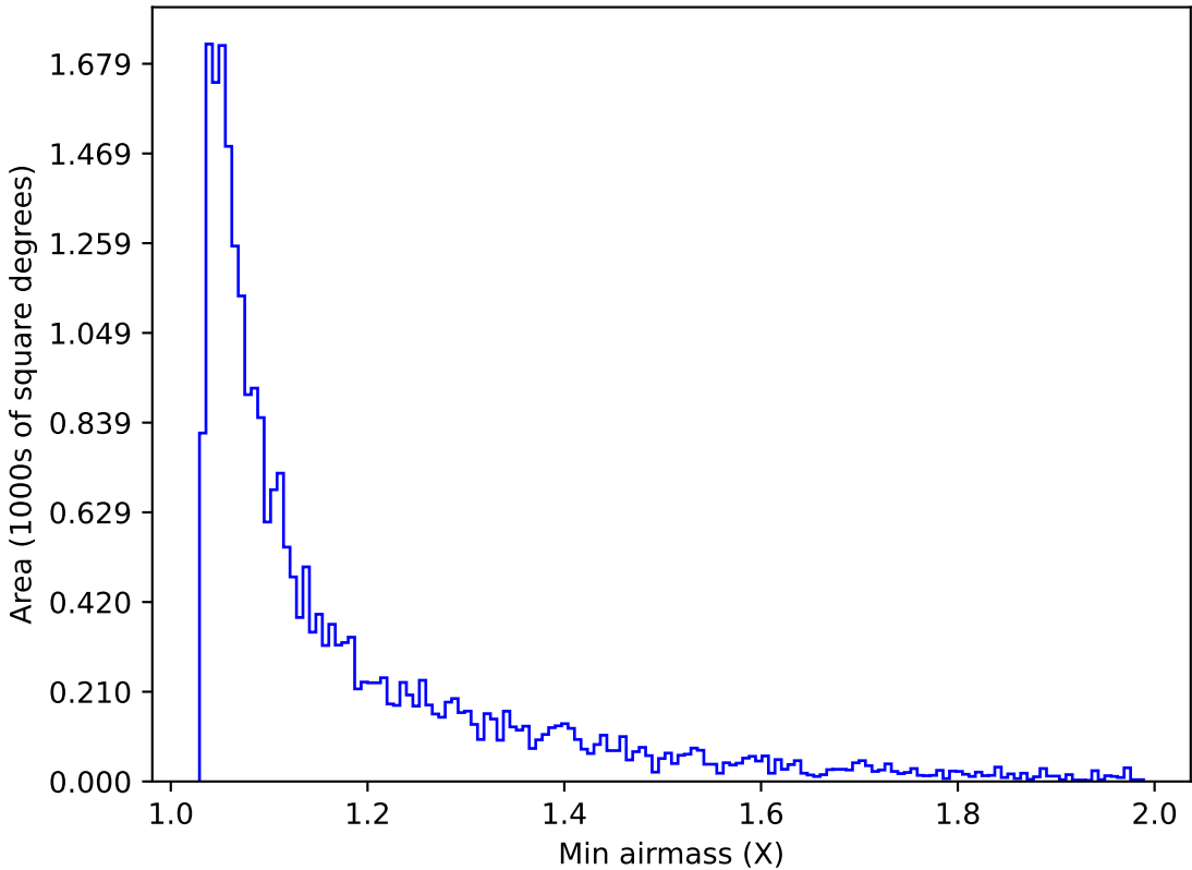
too_combined_no_nss_s10.0_v3.4_10yrs Yr 1 g band: Min airmass
