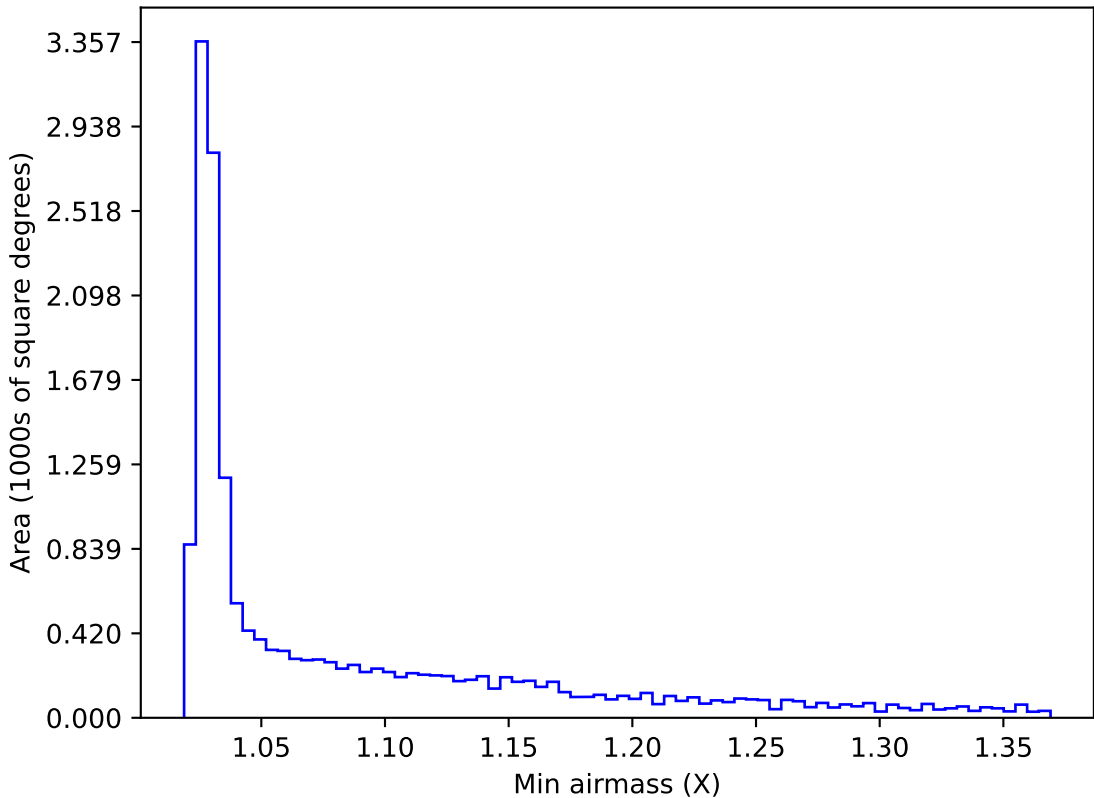
too_combined_no_nss_s10.0_v3.4_10yrs WFD z band: Min airmass
