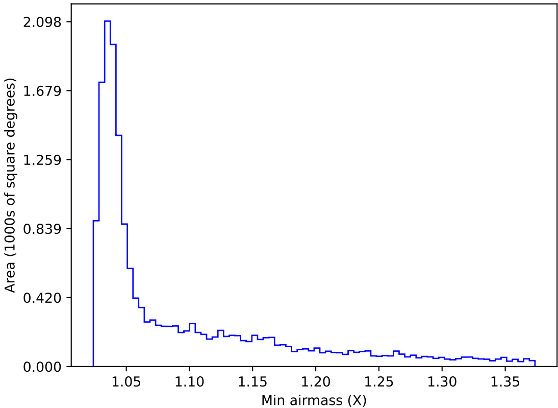
too_combined_no_nss_s10.0_v3.4_10yrs WFD u band: Min airmass
