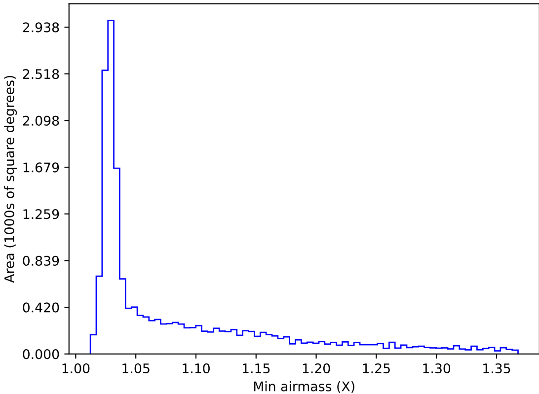
too_combined_no_nss_s10.0_v3.4_10yrs WFD i band: Min airmass
