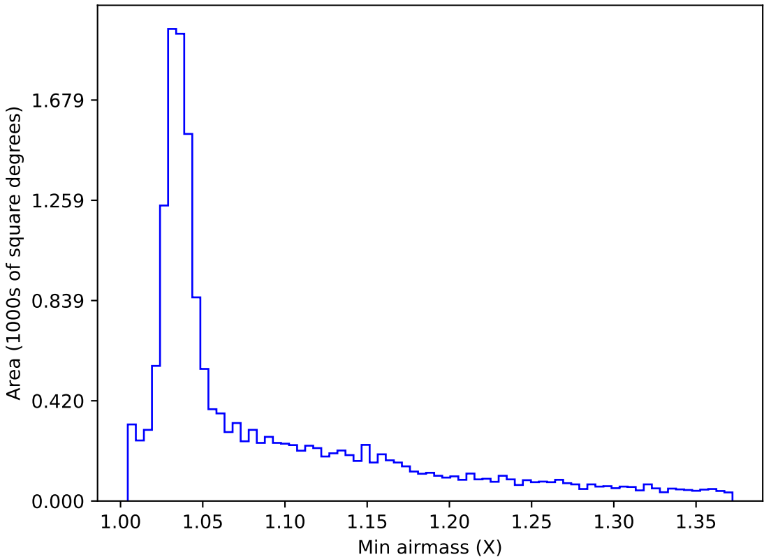
too_combined_no_nss_s10.0_v3.4_10yrs WFD g band: Min airmass
