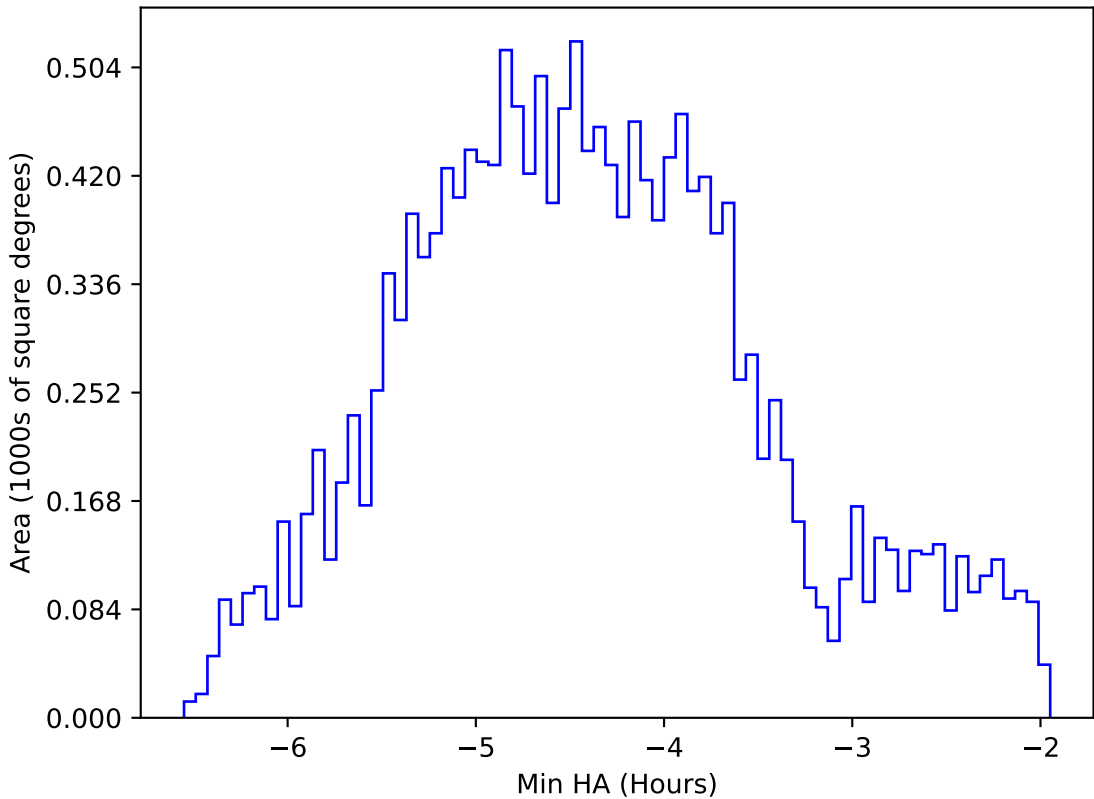
too_combined_no_nss_s10.0_v3.4_10yrs WFD z band: Min HA
