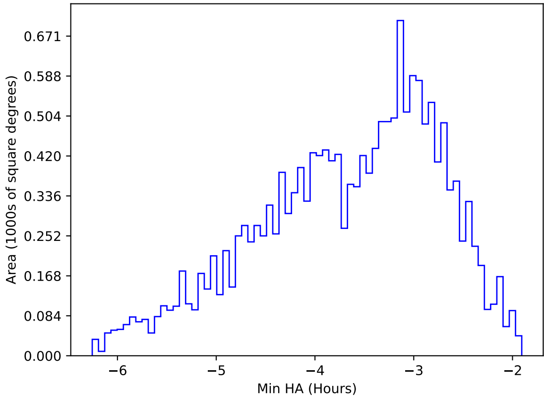
too_combined_no_nss_s10.0_v3.4_10yrs WFD y band: Min HA
