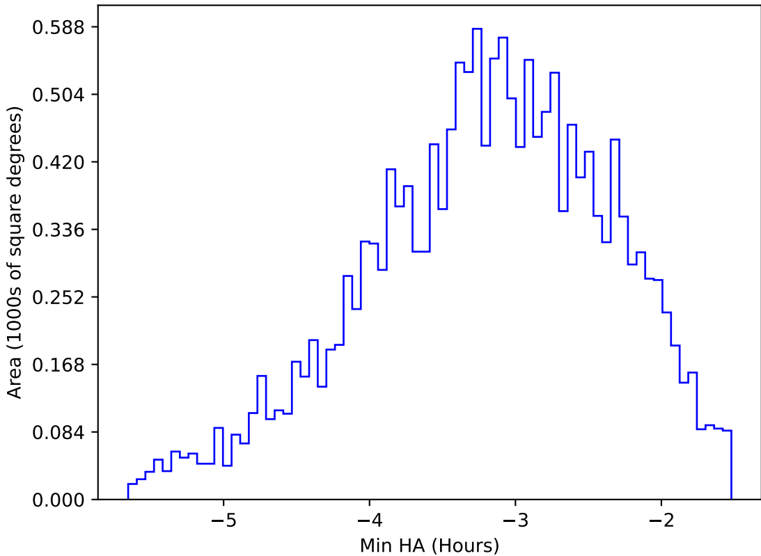
too_combined_no_nss_s10.0_v3.4_10yrs WFD u band: Min HA
