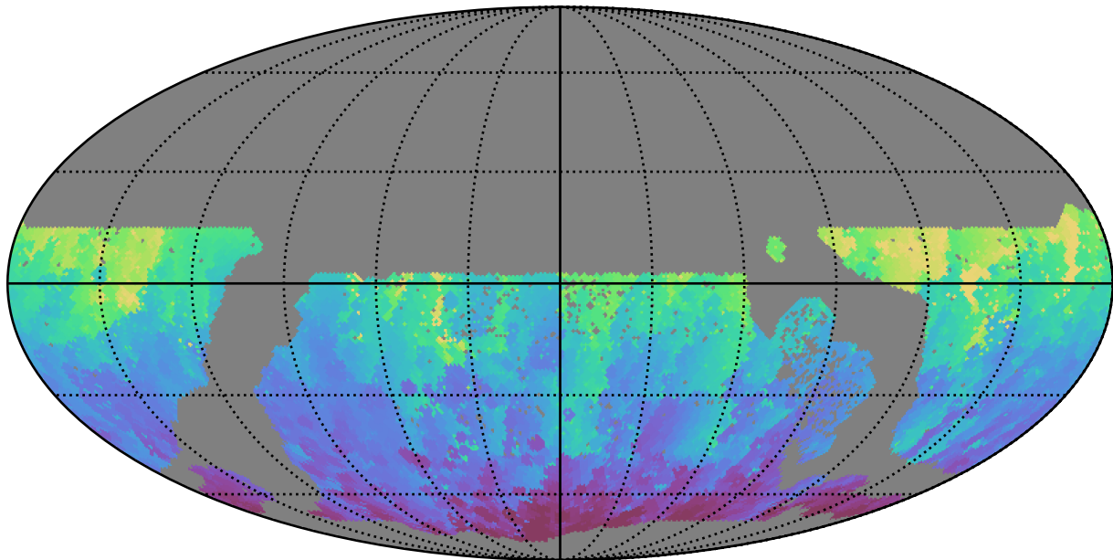
too_combined_no_nss_s10.0_v3.4_10yrs WFD g band: Min HA
