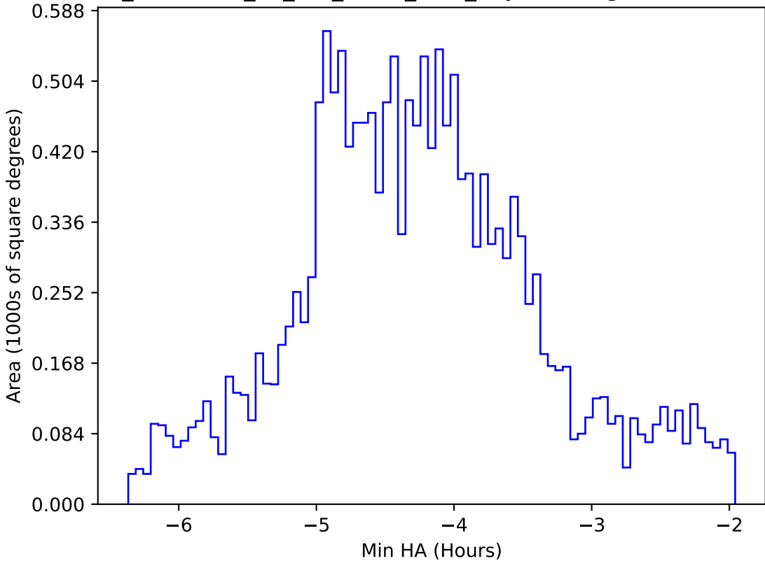
too_combined_no_nss_s10.0_v3.4_10yrs WFD g band: Min HA
