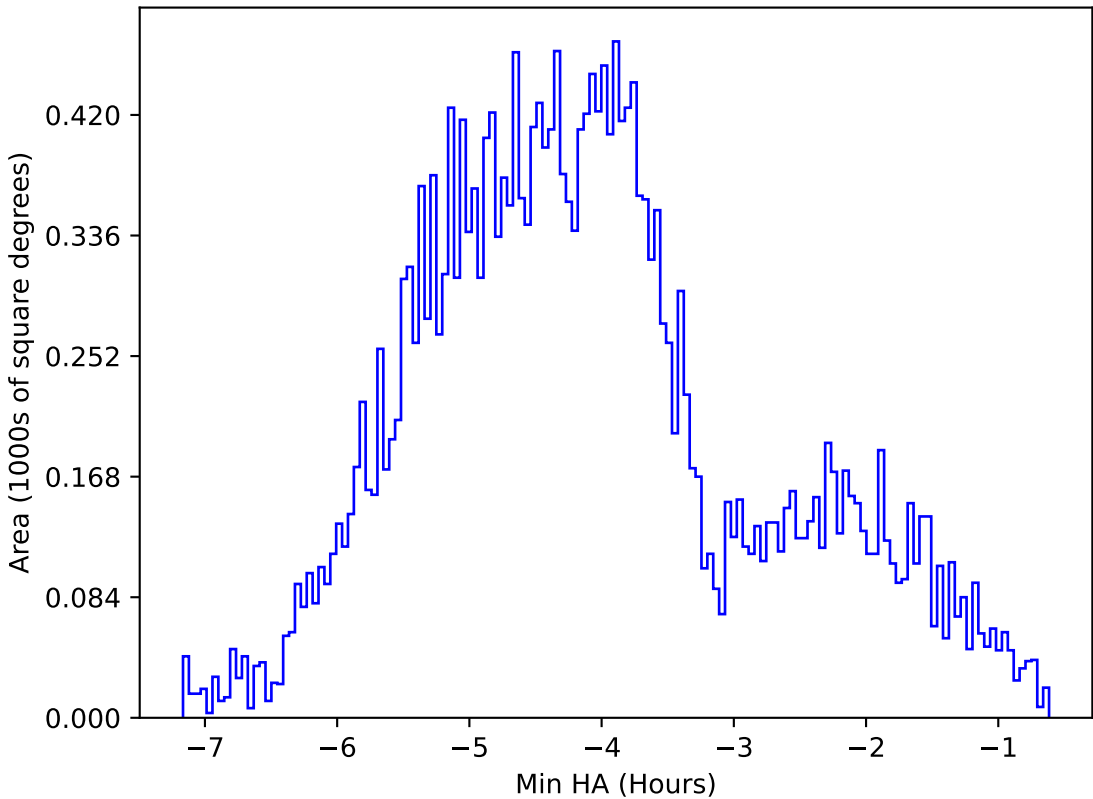
too_combined_no_nss_s10.0_v3.4_10yrs All sky z band: Min HA
