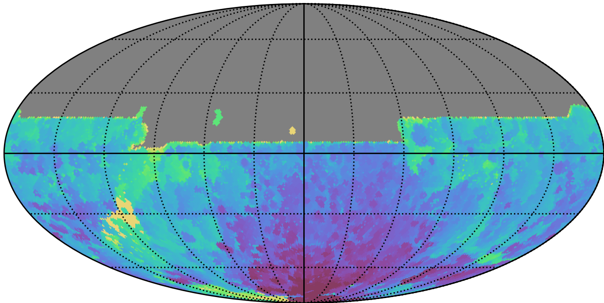
too_combined_no_nss_s10.0_v3.4_10yrs All sky y band: Min HA
