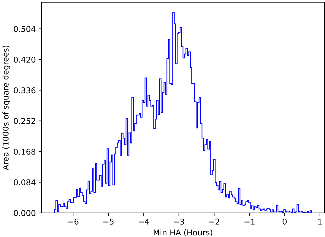
too_combined_no_nss_s10.0_v3.4_10yrs All sky y band: Min HA
