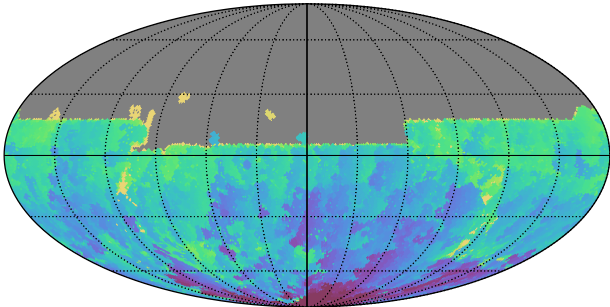
too_combined_no_nss_s10.0_v3.4_10yrs All sky u band: Min HA
