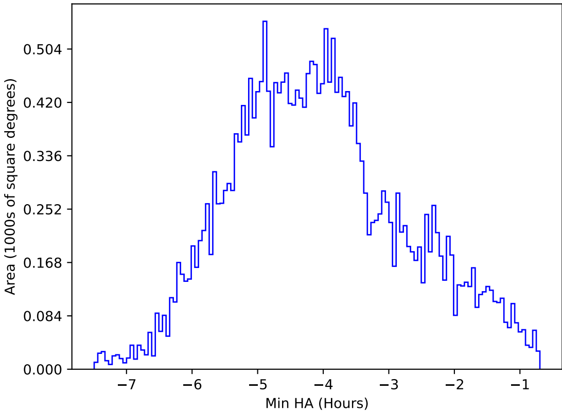
too_combined_no_nss_s10.0_v3.4_10yrs All sky i band: Min HA
