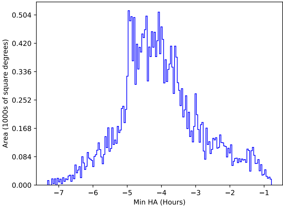
too_combined_no_nss_s10.0_v3.4_10yrs All sky g band: Min HA
