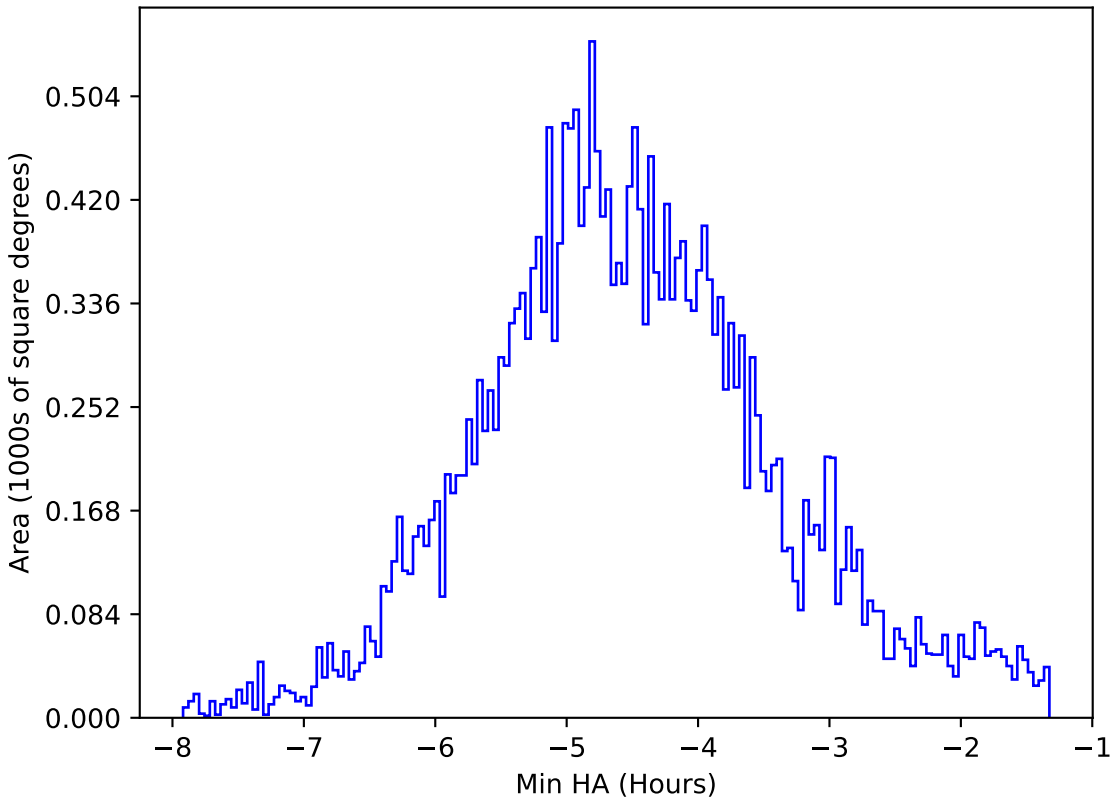
too_combined_no_nss_s10.0_v3.4_10yrs All sky all bands: Min HA
