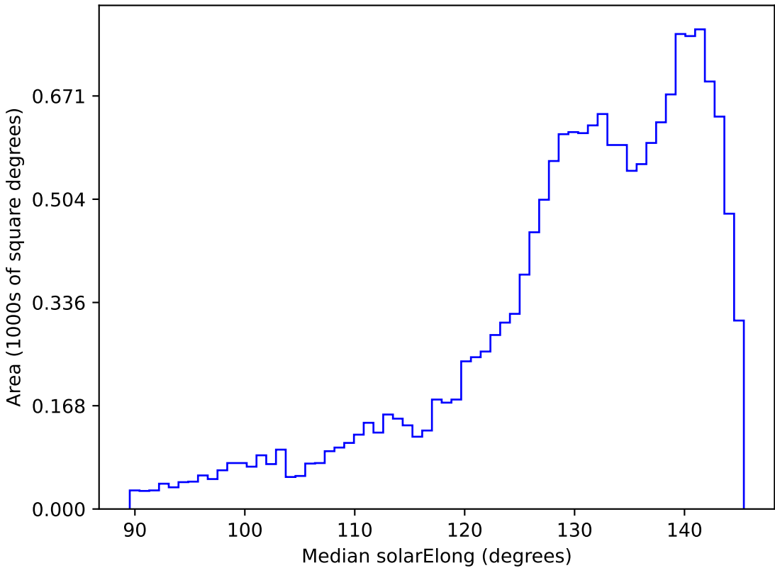
too_combined_no_nss_s10.0_v3.4_10yrs WFD all bands: Median solarElong
