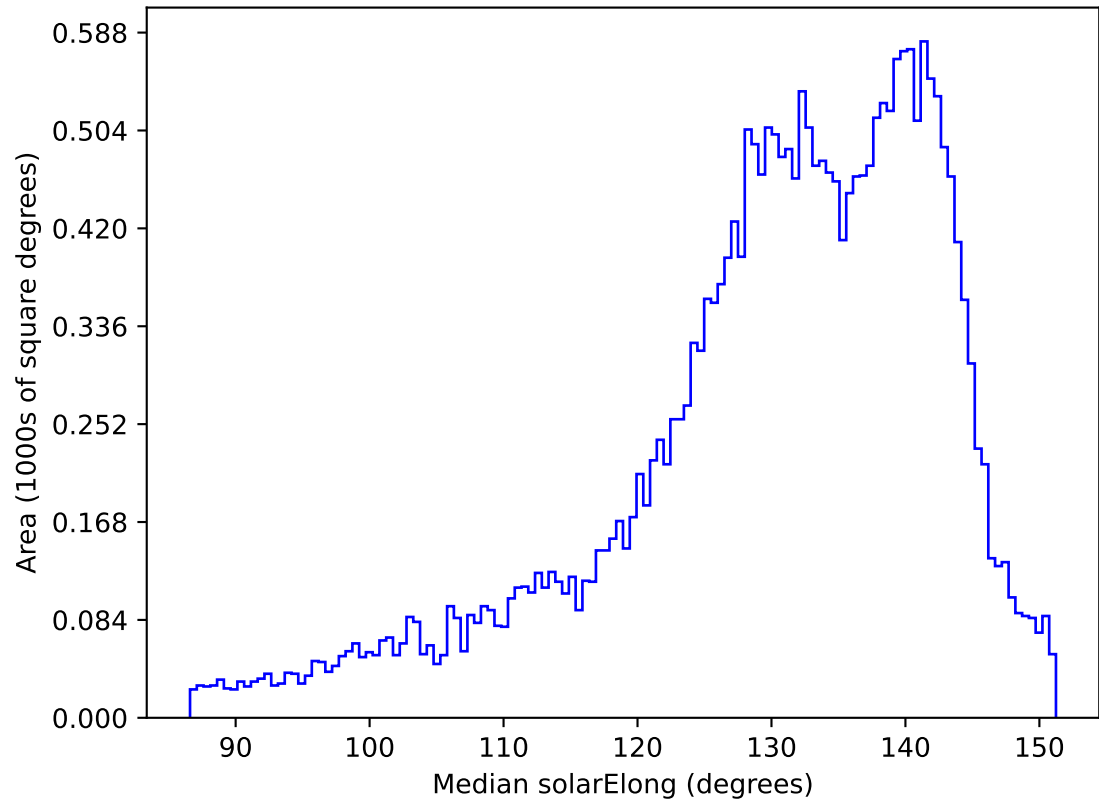
too_combined_no_nss_s10.0_v3.4_10yrs All sky all bands: Median solarElong
