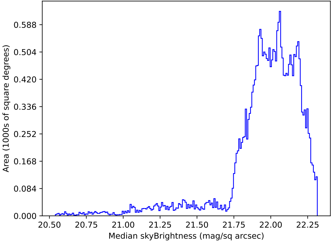
too_combined_no_nss_s10.0_v3.4_10yrs Yr 1 g band: Median skyBrightness
