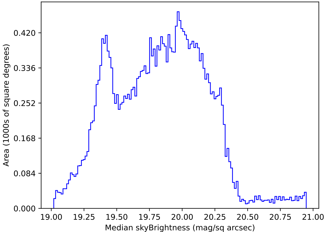
too_combined_no_nss_s10.0_v3.4_10yrs Yr 1 all bands: Median skyBrightness
