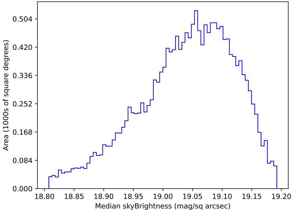
too_combined_no_nss_s10.0_v3.4_10yrs WFD z band: Median skyBrightness
