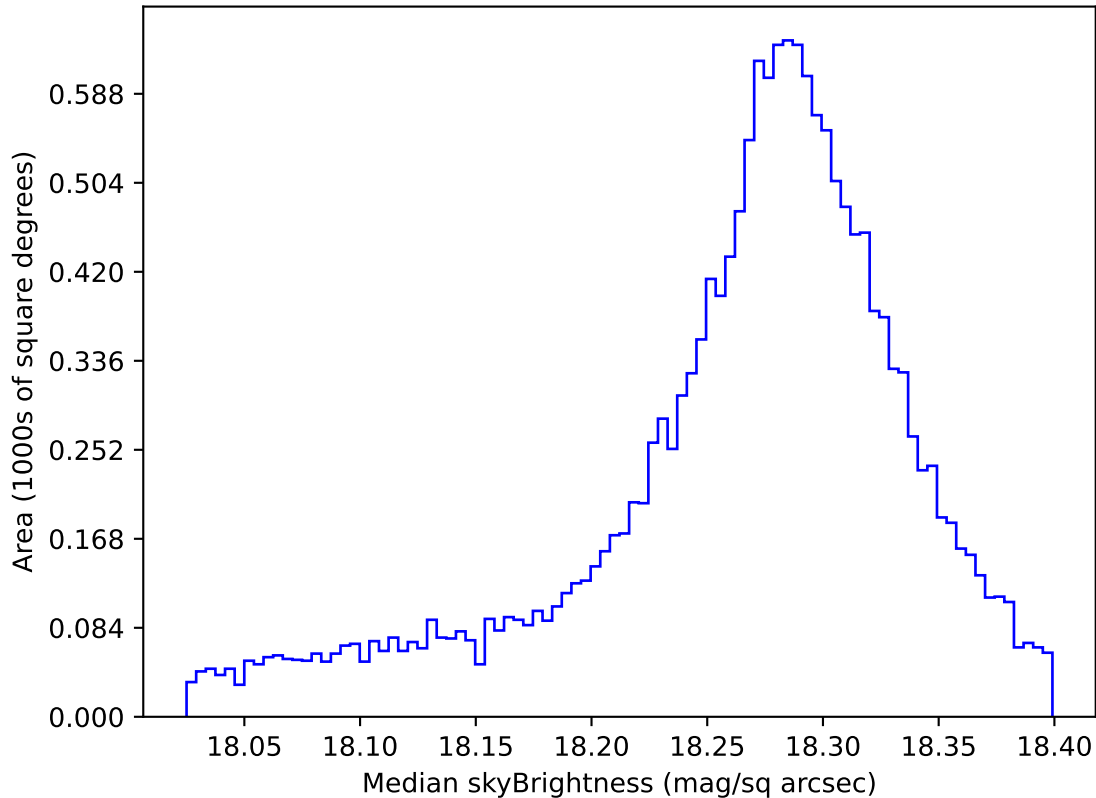
too_combined_no_nss_s10.0_v3.4_10yrs WFD y band: Median skyBrightness
