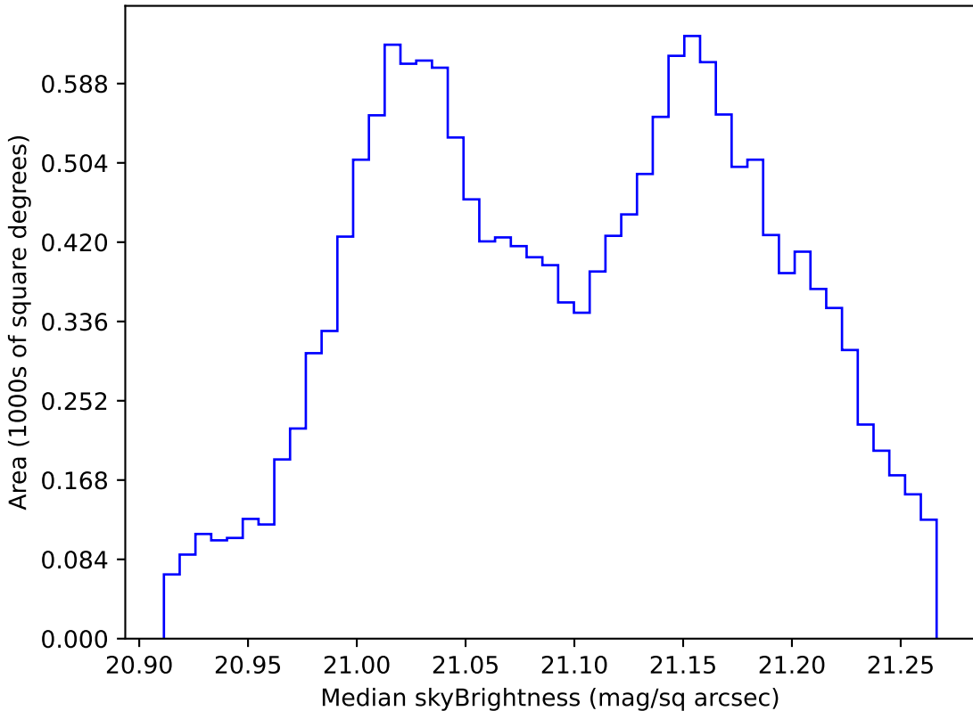
too_combined_no_nss_s10.0_v3.4_10yrs WFD r band: Median skyBrightness
