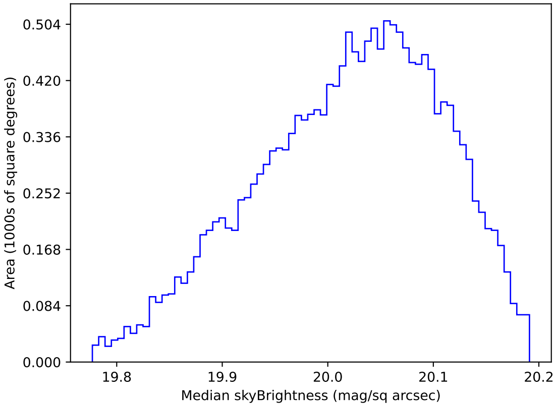
too_combined_no_nss_s10.0_v3.4_10yrs WFD i band: Median skyBrightness
