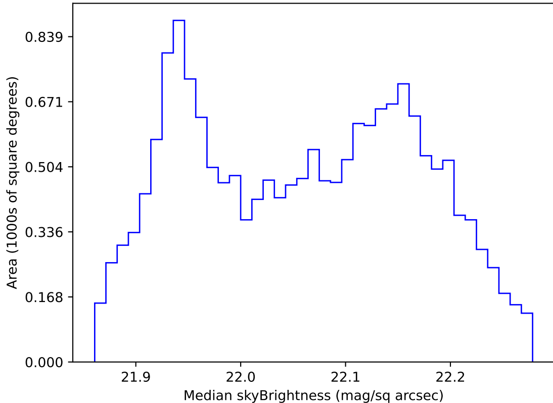
too_combined_no_nss_s10.0_v3.4_10yrs WFD g band: Median skyBrightness
