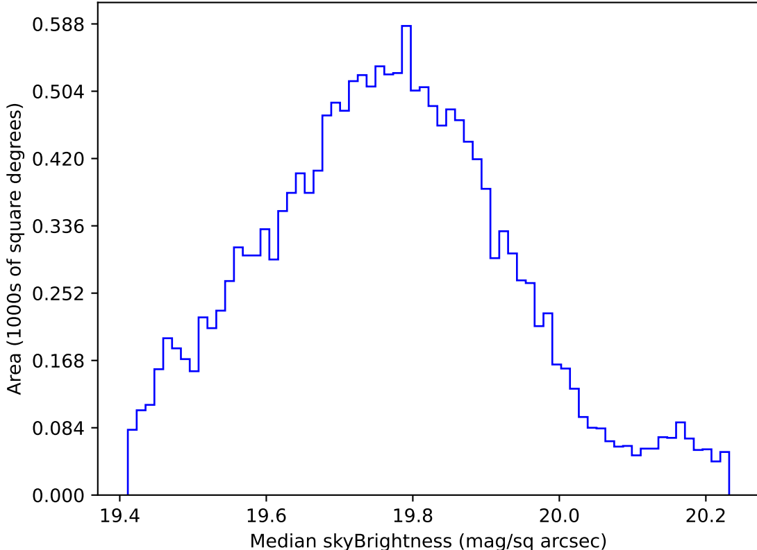
too_combined_no_nss_s10.0_v3.4_10yrs WFD all bands: Median skyBrightness
