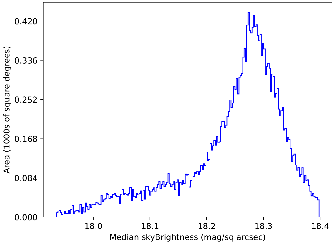
too_combined_no_nss_s10.0_v3.4_10yrs All sky y band: Median skyBrightness
