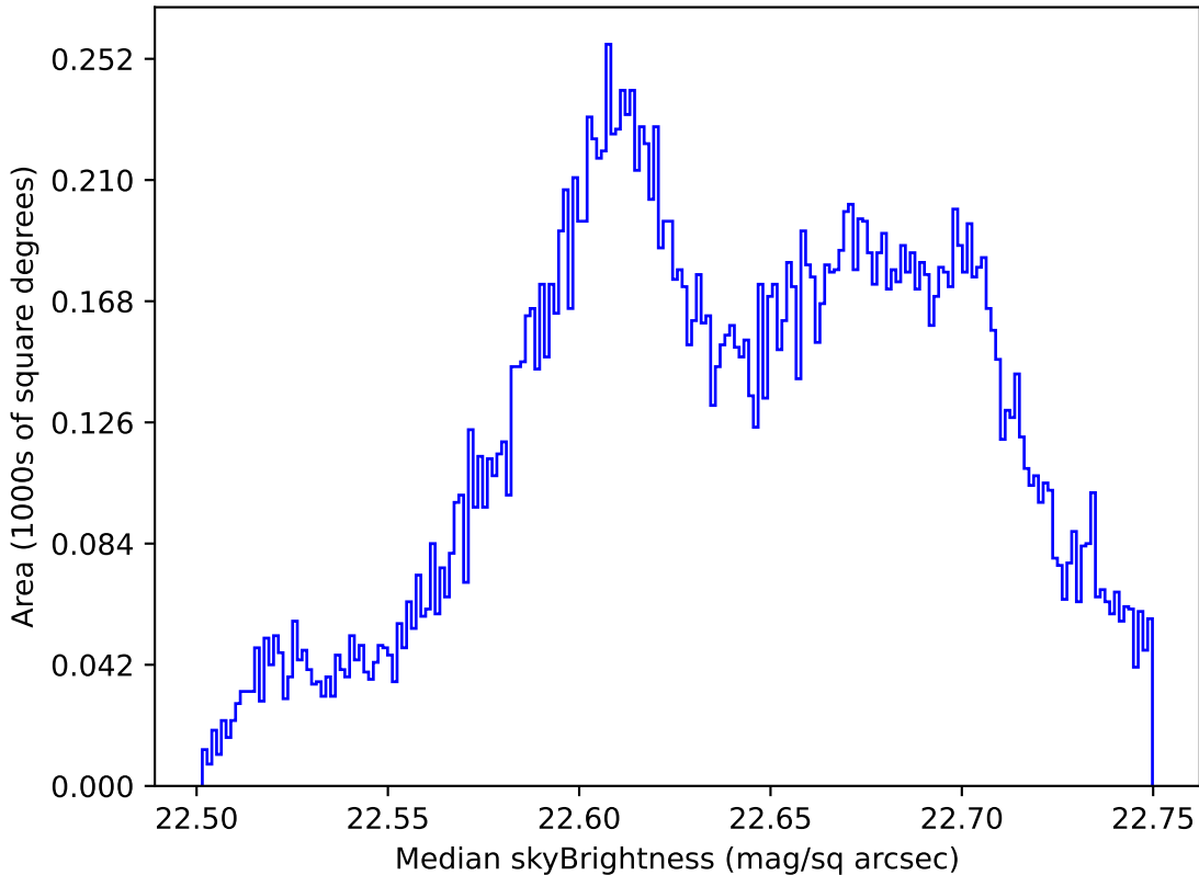
too_combined_no_nss_s10.0_v3.4_10yrs All sky u band: Median skyBrightness
