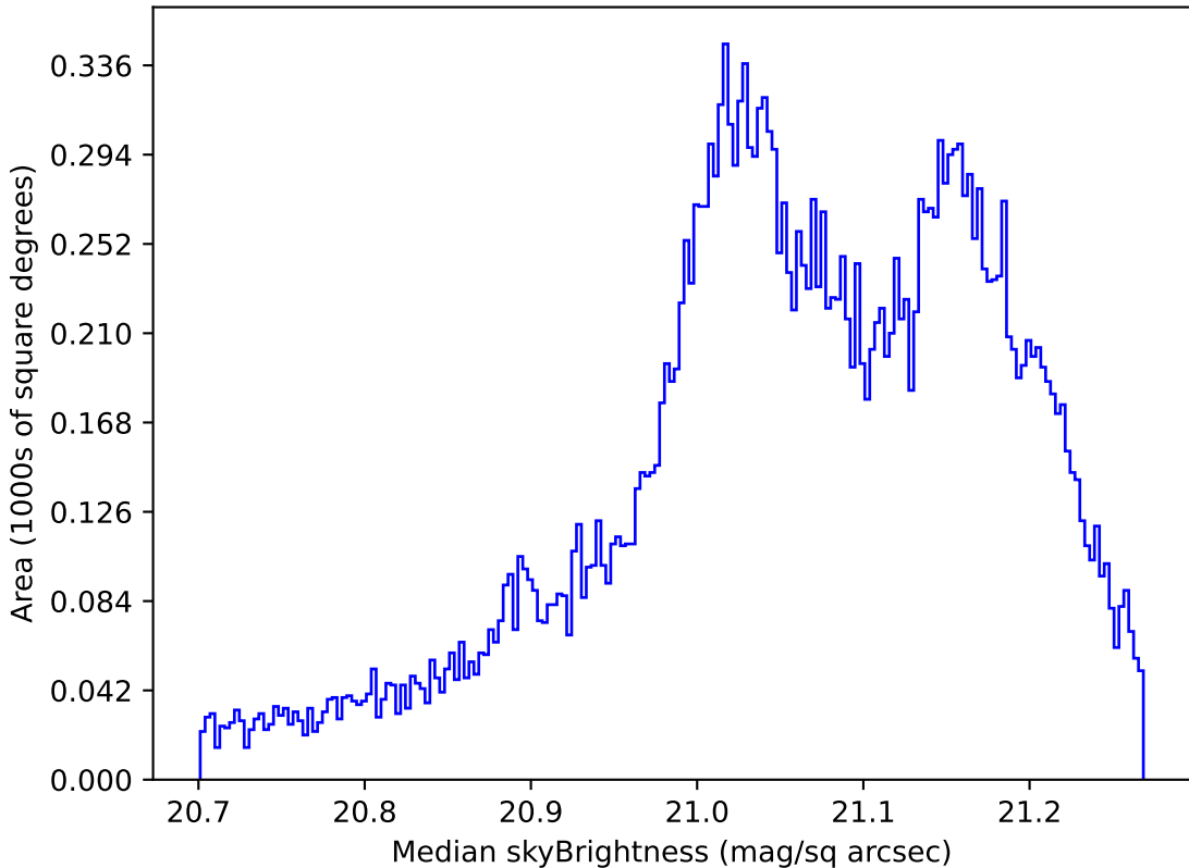
too_combined_no_nss_s10.0_v3.4_10yrs All sky r band: Median skyBrightness
