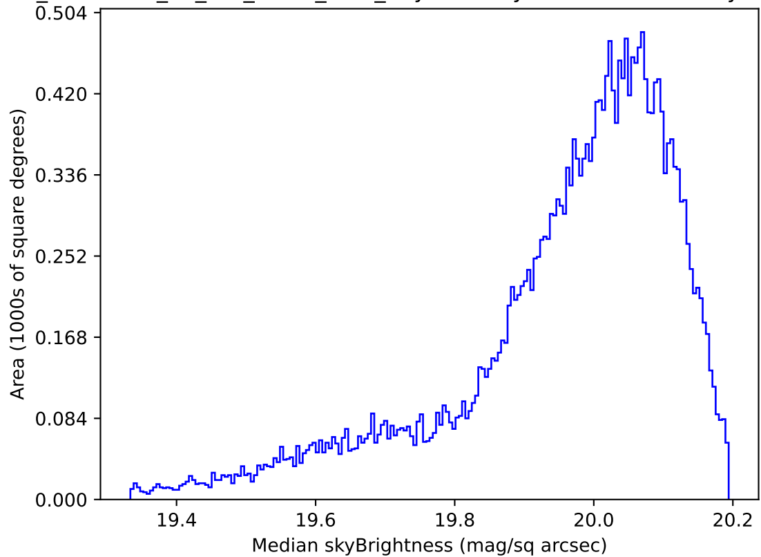
too_combined_no_nss_s10.0_v3.4_10yrs All sky i band: Median skyBrightness
