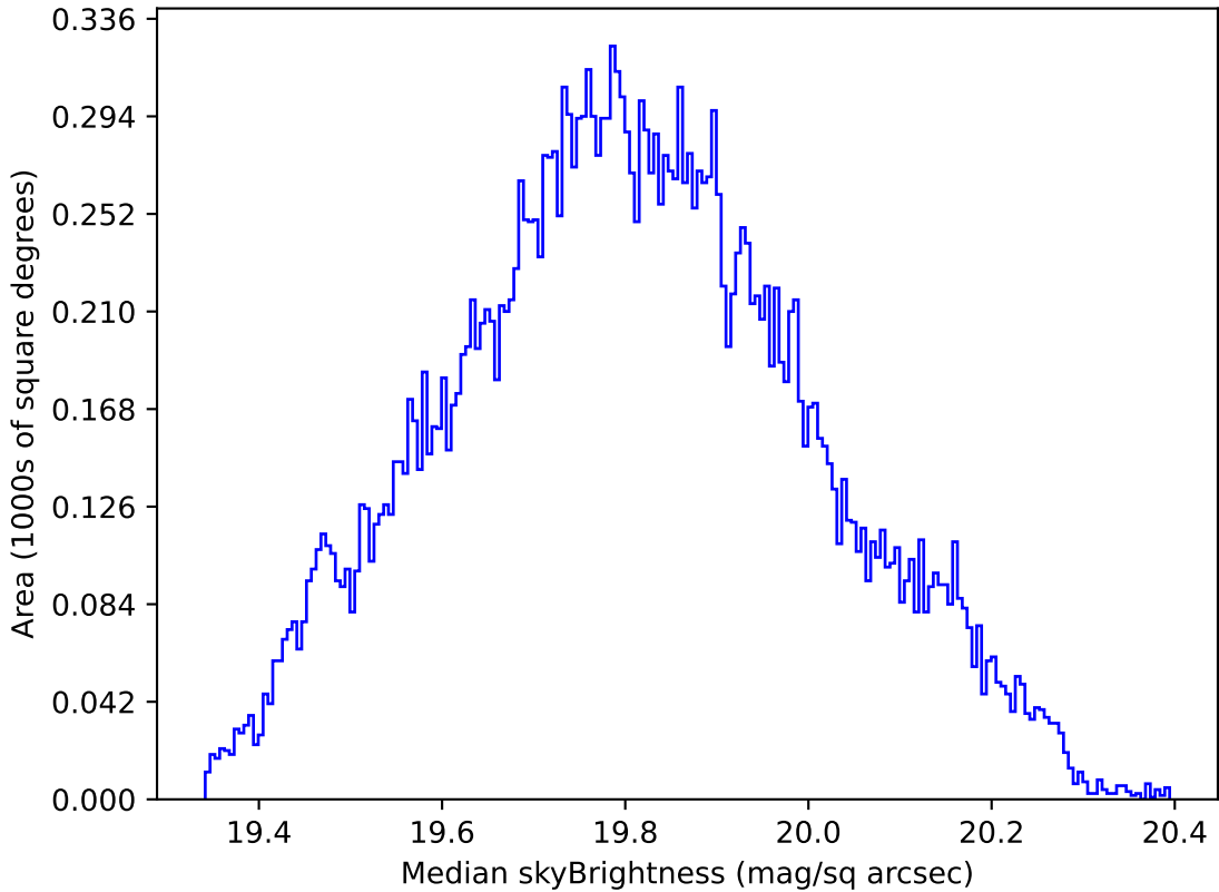
too_combined_no_nss_s10.0_v3.4_10yrs All sky all bands: Median skyBrightness
