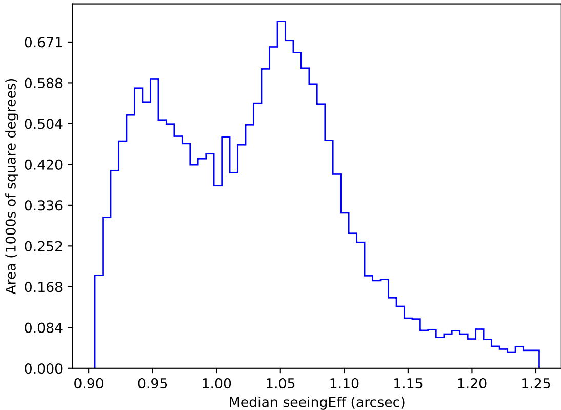
too_combined_no_nss_s10.0_v3.4_10yrs WFD all bands: Median seeingEff
