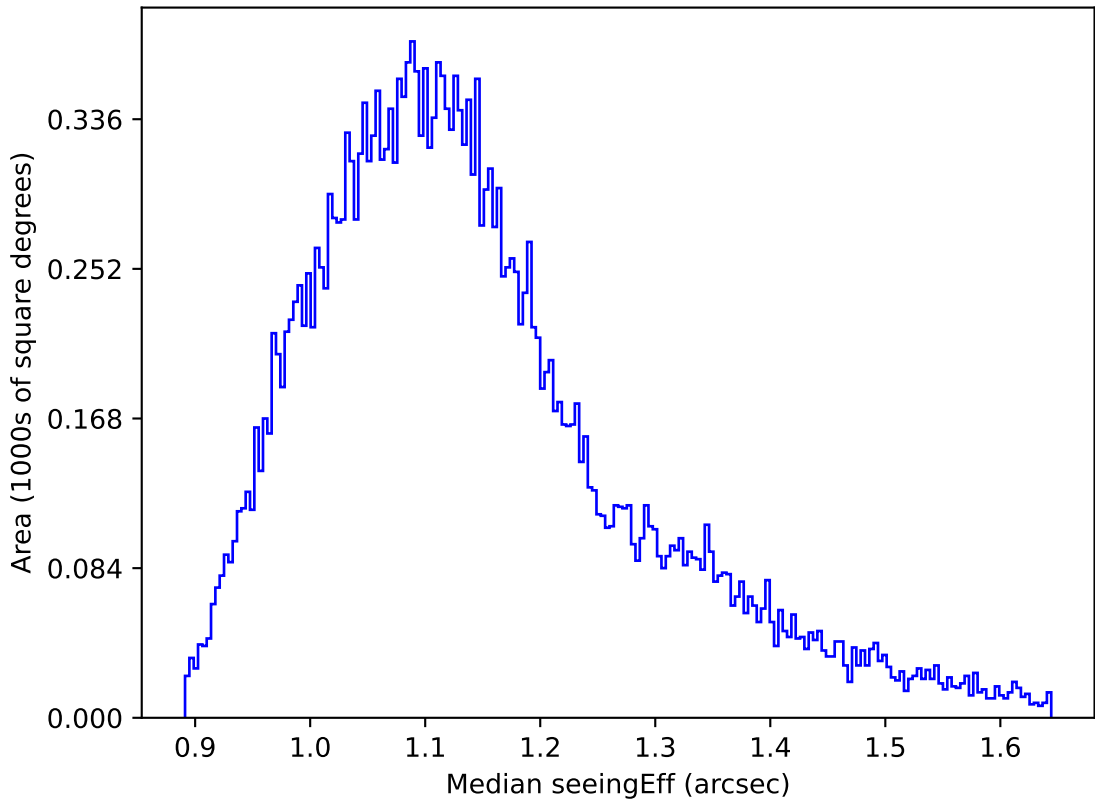
too_combined_no_nss_s10.0_v3.4_10yrs All sky g band: Median seeingEff
