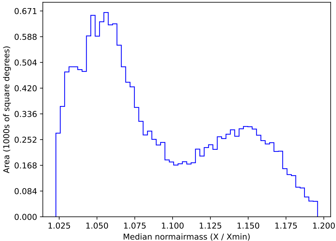
too_combined_no_nss_s10.0_v3.4_10yrs WFD z band: Median normairmass
