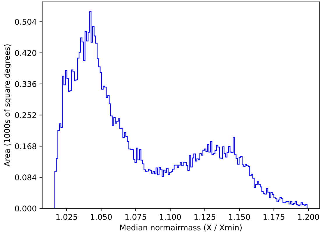
too_combined_no_nss_s10.0_v3.4_10yrs All sky i band: Median normairmass
