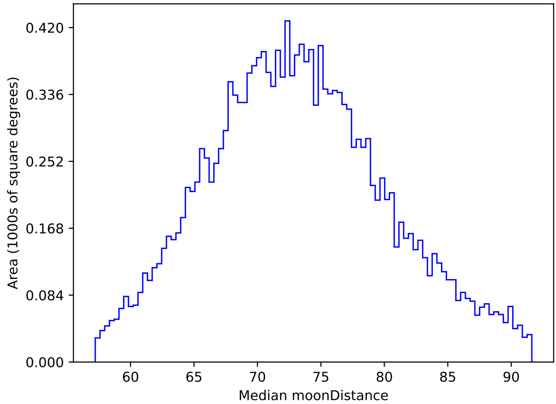
too_combined_no_nss_s10.0_v3.4_10yrs WFD z band: Median moonDistance
