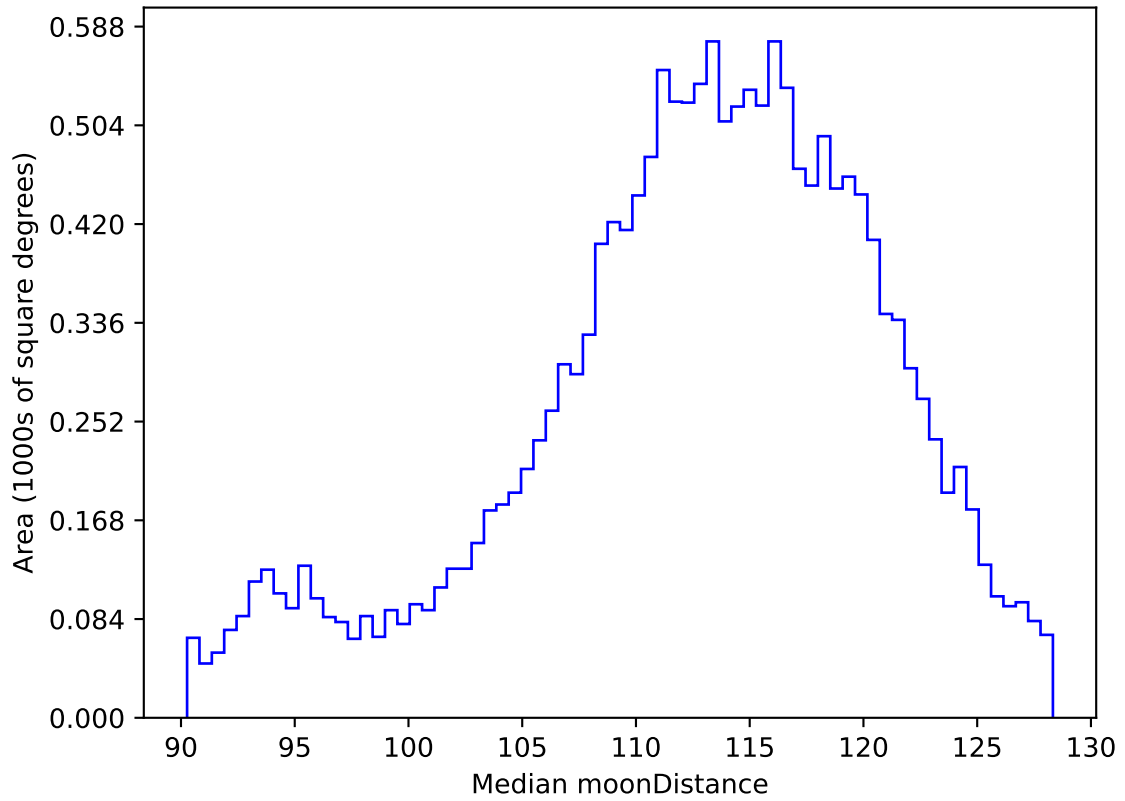
too_combined_no_nss_s10.0_v3.4_10yrs WFD r band: Median moonDistance
