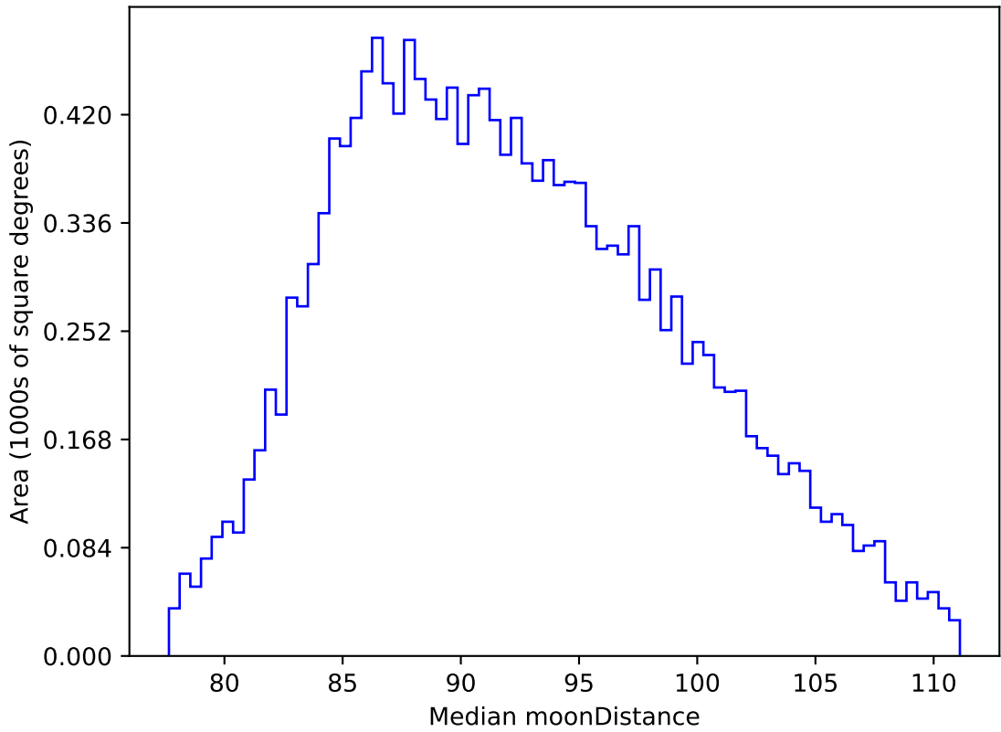
too_combined_no_nss_s10.0_v3.4_10yrs WFD i band: Median moonDistance
