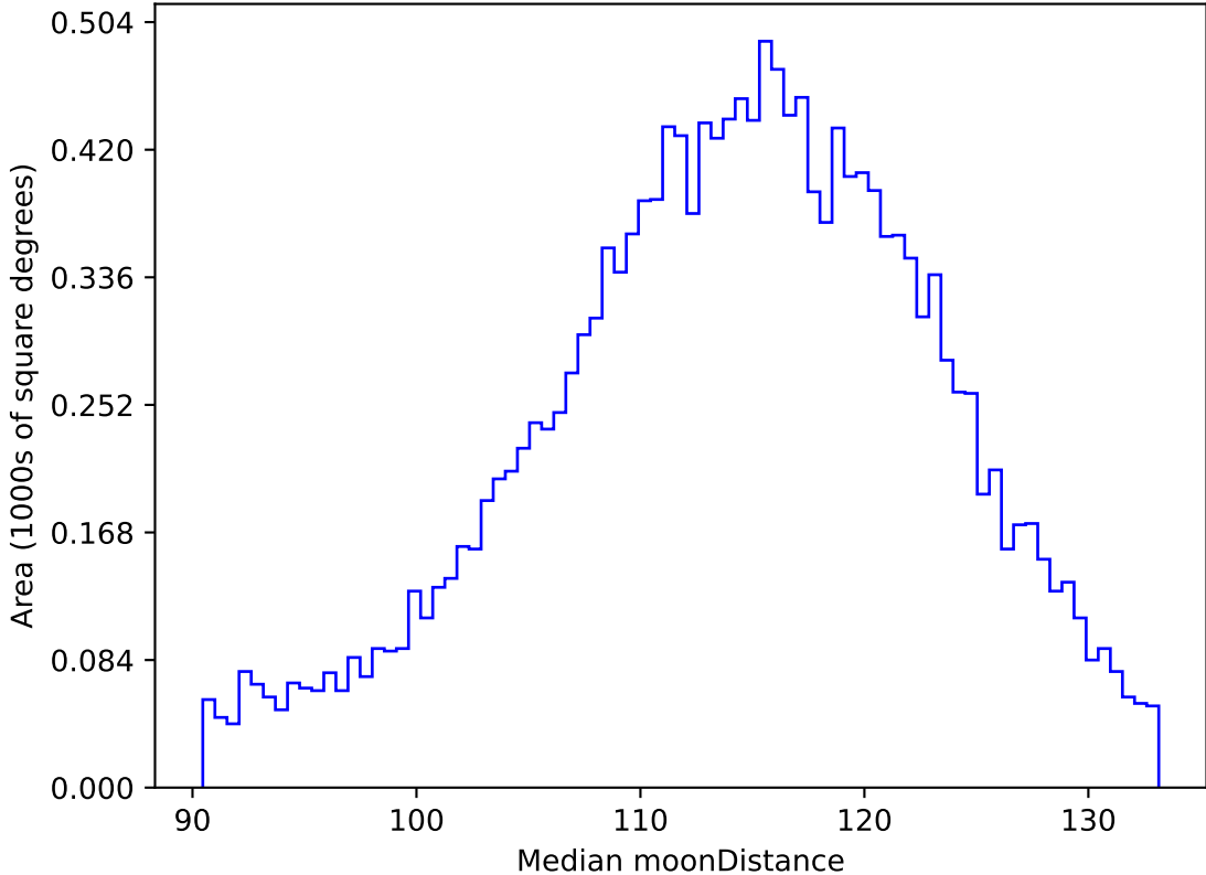
too_combined_no_nss_s10.0_v3.4_10yrs WFD g band: Median moonDistance
