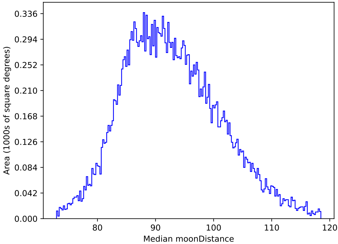
too_combined_no_nss_s10.0_v3.4_10yrs All sky i band: Median moonDistance
