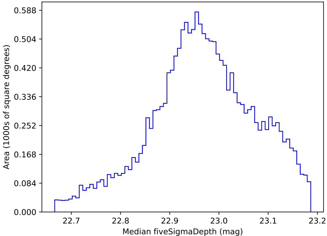
too_combined_no_nss_s10.0_v3.4_10yrs WFD z band: Median fiveSigmaDepth
