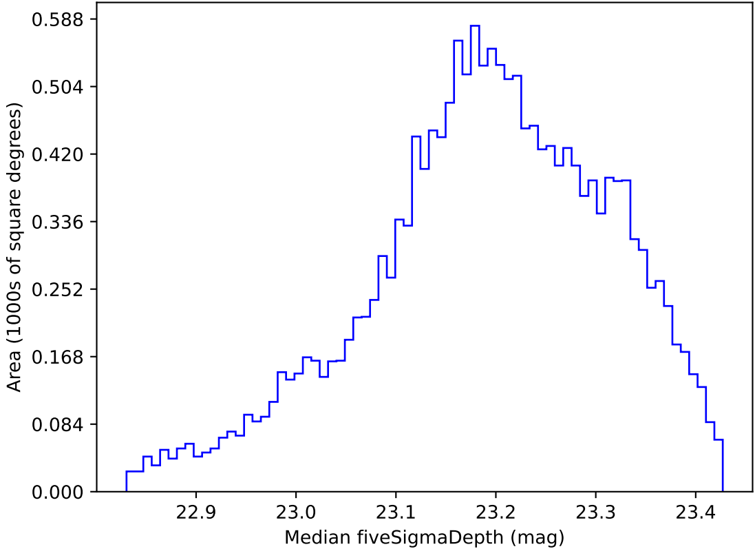
too_combined_no_nss_s10.0_v3.4_10yrs WFD u band: Median fiveSigmaDepth
