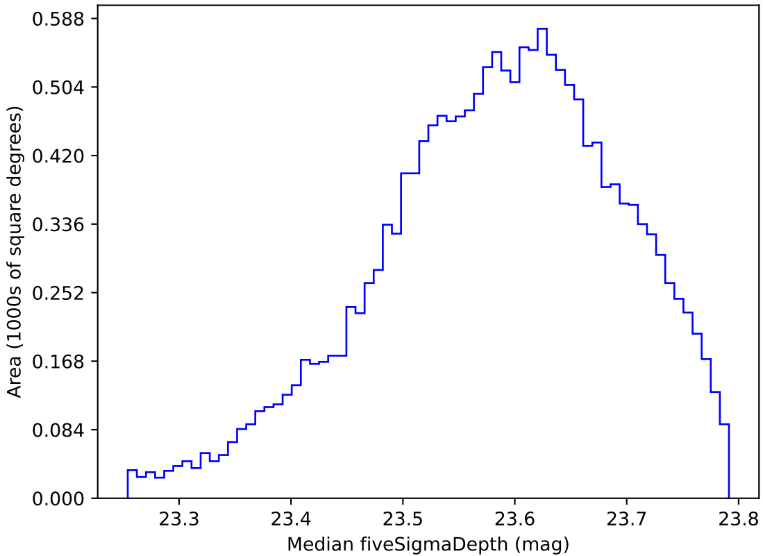
too_combined_no_nss_s10.0_v3.4_10yrs WFD i band: Median fiveSigmaDepth
