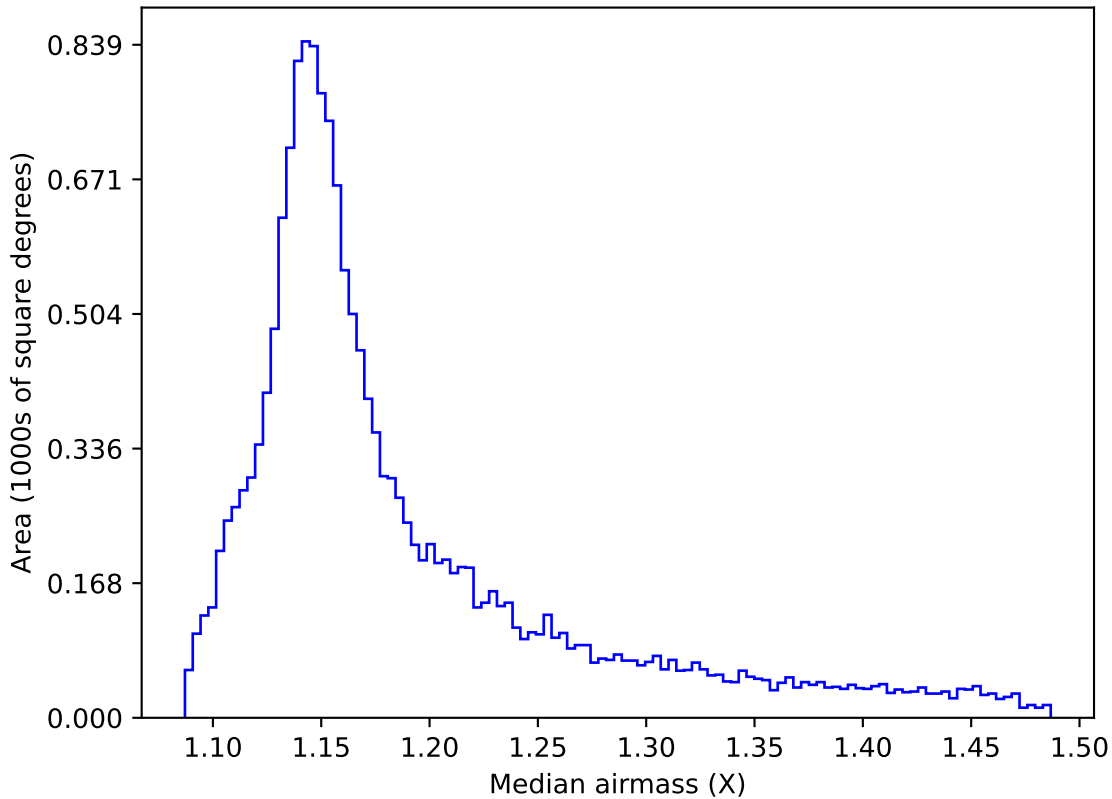
too_combined_no_nss_s10.0_v3.4_10yrs WFD y band: Median airmass
