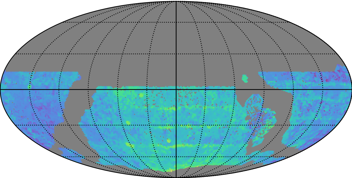
too_combined_no_nss_s10.0_v3.4_10yrs WFD y band: Median Season Length
