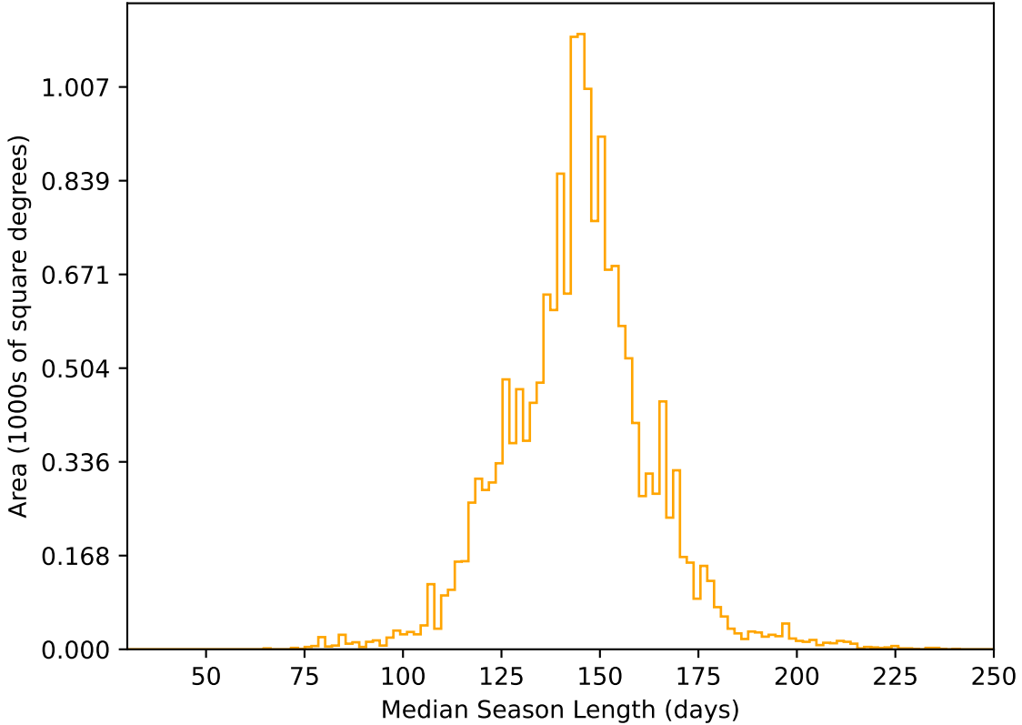
too_combined_no_nss_s10.0_v3.4_10yrs WFD r band: Median Season Length
