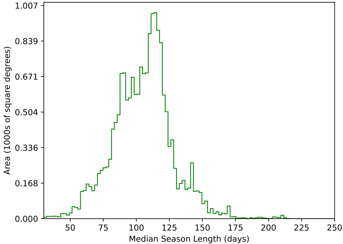
too_combined_no_nss_s10.0_v3.4_10yrs WFD g band: Median Season Length
