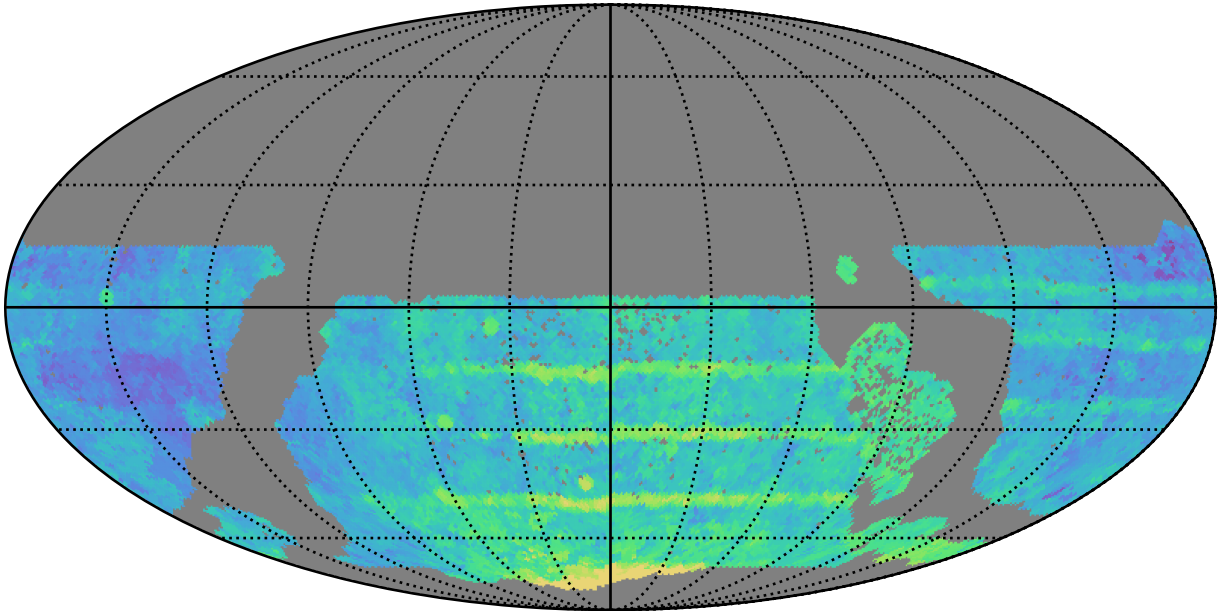
too_combined_no_nss_s10.0_v3.4_10yrs WFD all bands: Median Season Length
