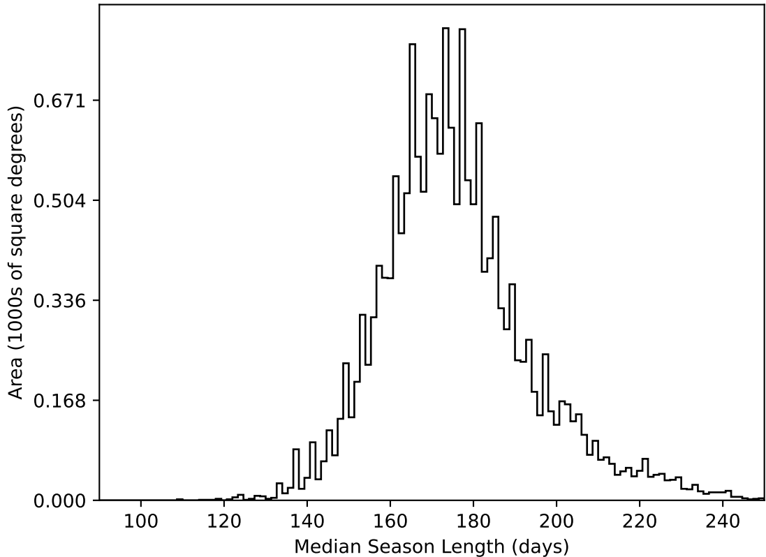
too_combined_no_nss_s10.0_v3.4_10yrs WFD all bands: Median Season Length
